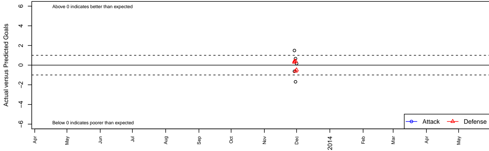
Strikers FC Whittier –Unk B95 Dots are actual minus expected GF (blue circles) and GA (red triangles). Blue line is smoothed change in attack strength. Red is smoothed change in defense strength.
